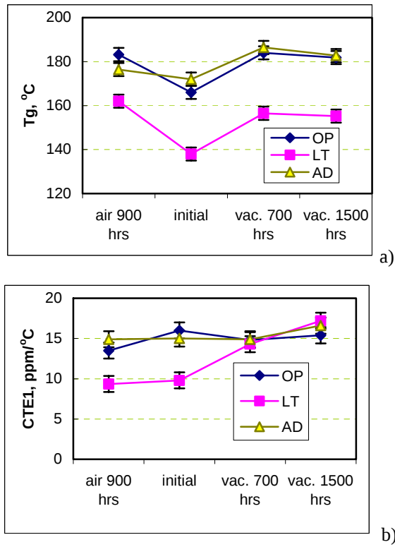
Figure 9. Effect of vacuum and air storage at 210 °C on the glass transition temperatures (a) and coefficients of temperature expansion in a glassy state (b) of molding compounds.
