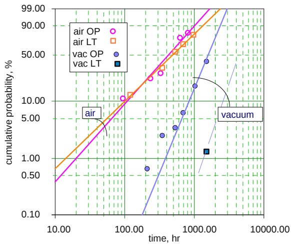
Figure 4. Cumulative probability for wire bond failures ( R_c > 10 Ohm) during storage of OP and LT parts in air and vacuum chambers.
