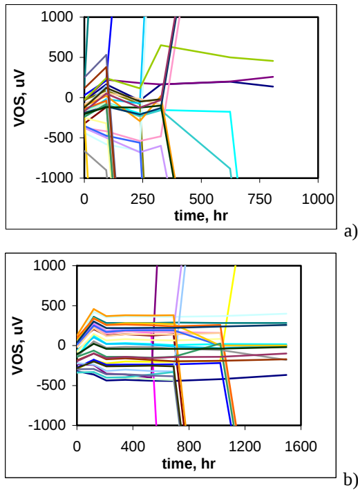
Figure 6. Variations of the offset voltages for operational amplifiers during high temperature storage testing in air (a) and vacuum (b) chambers.
