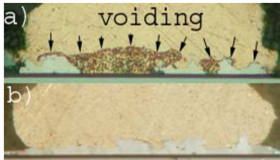
Figure 13. Cross section of wire bonds after 700 hrs. aging in air (a) and in vacuum (b). Note that extensive voiding in Au/Al intermetallic layers were observed only in the parts aged in air.
