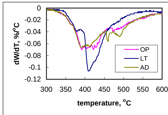
Figure 1. Differential TGA curves of the three plastic packages used.
