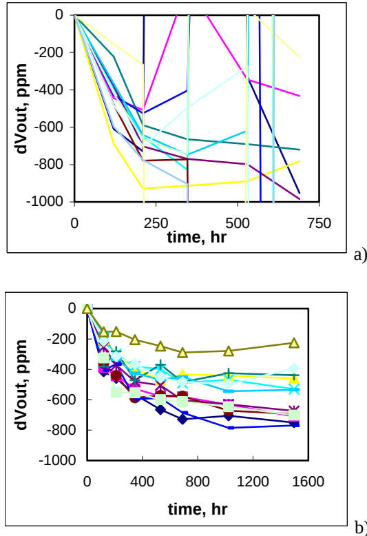
Figure 7. Output deviations of precision voltage reference microcircuits (LT) during HTS testing in air (a) and vacuum (b) chambers.
