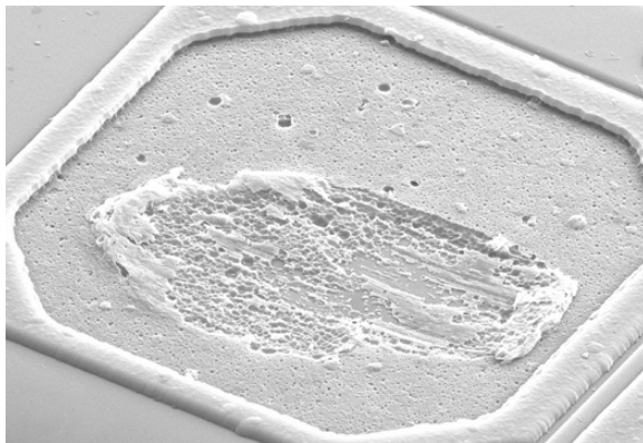
Figure 16. An example of corrosion of Al on an unbonded contact pad with a probe mark in the LT microcircuits after 1500 hrs at 210 °C in vacuum chamber.
